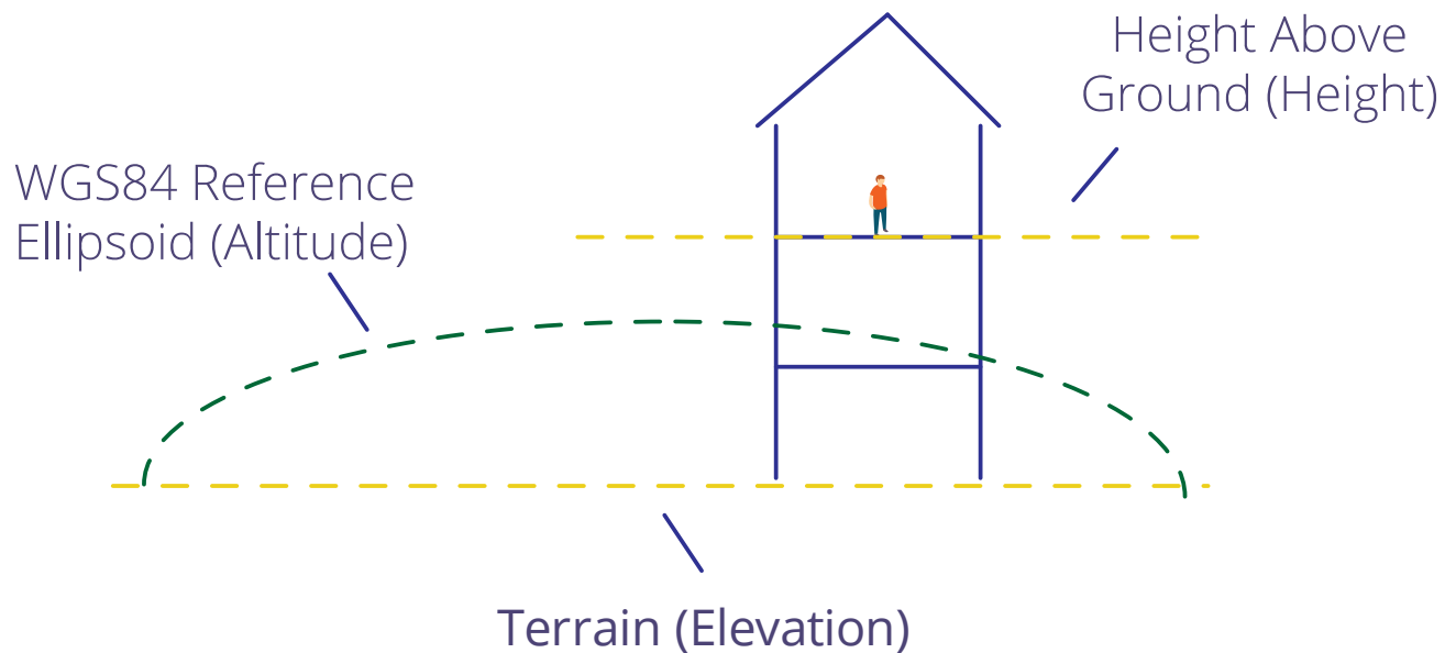
Figure 6: Terrain, Ellipsoid, and AGL
