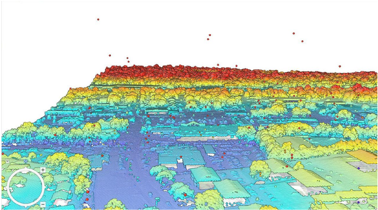
Figure 25: Raw LiDAR for Jefferson City Area (Oblique view) 44
