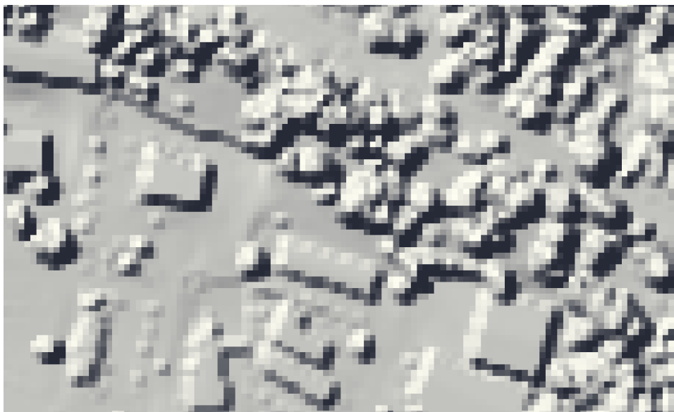
Figure 38: DSM for Jefferson City Area resampled from 30 inch pixels to 10 foot pixels with Hillshade
