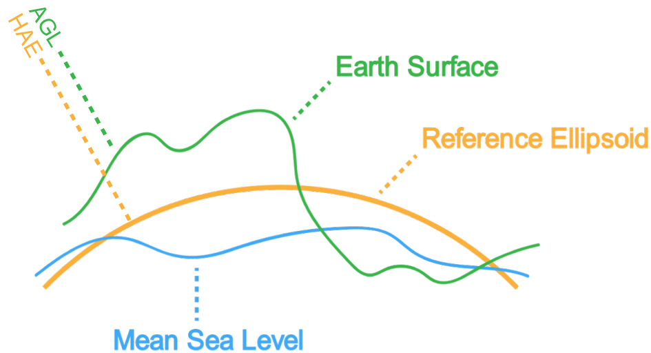
Figure 5: Relationship Between the Earth's Surface, a Reference Ellipsoid, Mean Sea Level, AGL, and HAE
