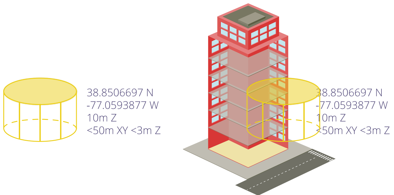
Figure 8: 3D Geodetic Location (left) and 3D Geodetic Location with a 3D Map (Right)
