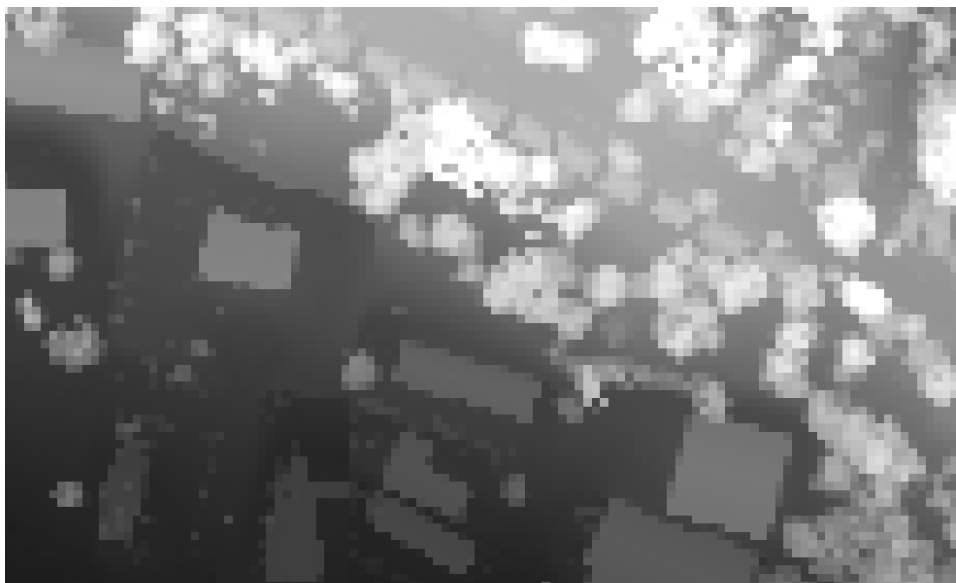
Figure 36: DSM for Jefferson City Area resampled from 30 inch pixels to 10 foot pixels
